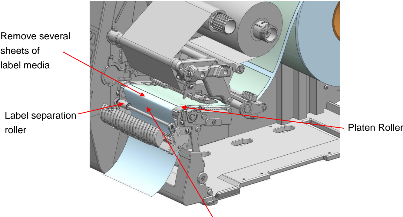
Insert media between platen roller and label separation roller
