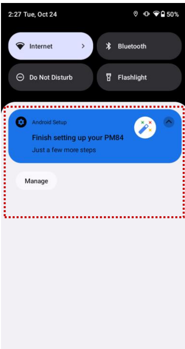
Figure 24 Notification panel
