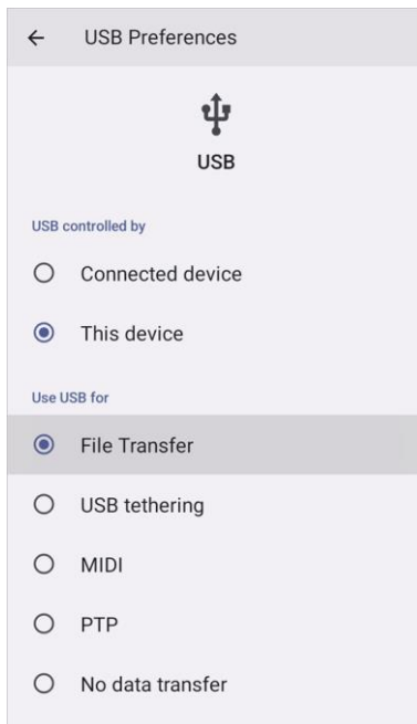
Figure 42 USB Preferences
