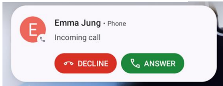
Figure 35 Receiving call
