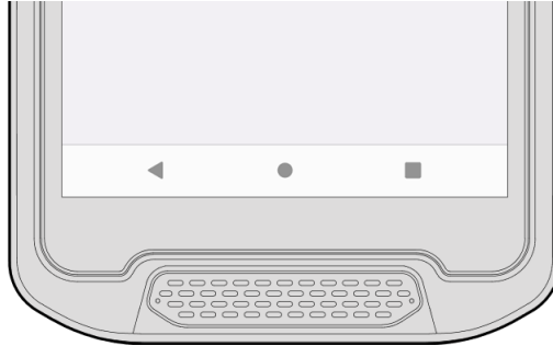
Figure 19 Navigation bar
