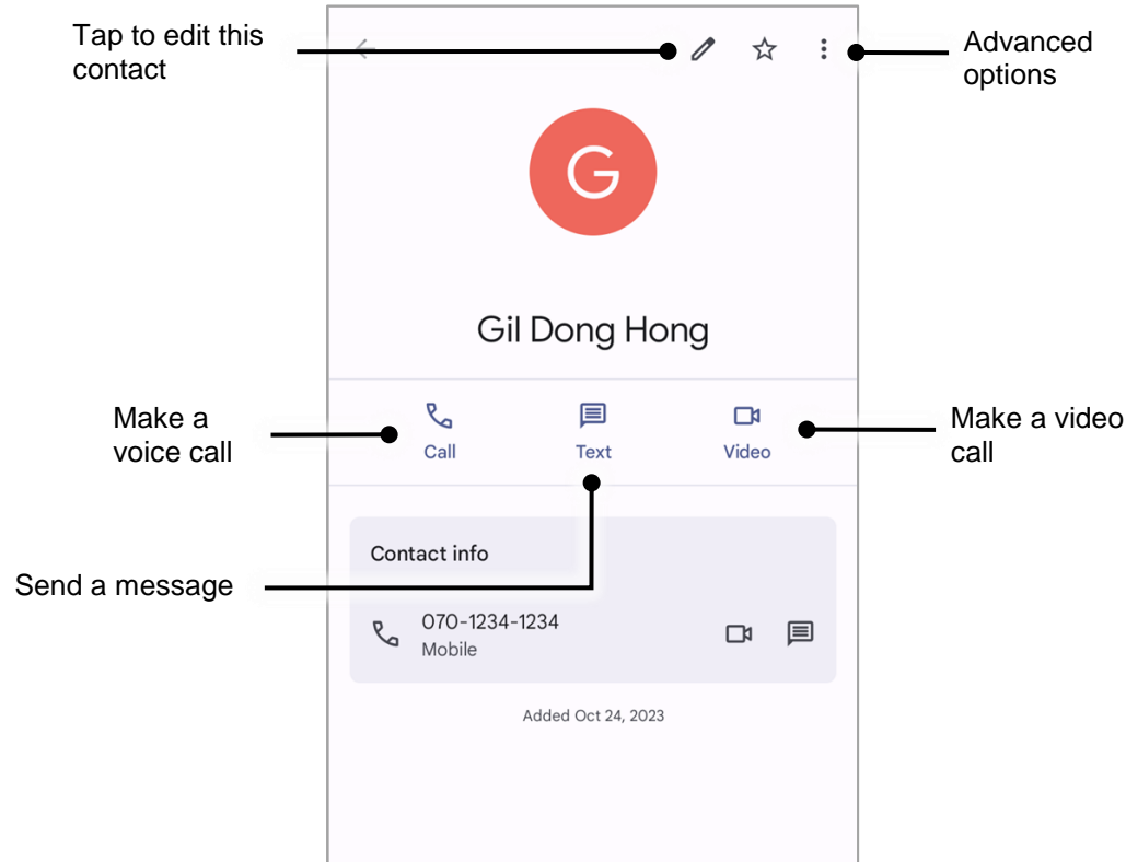
Figure 37 Contact detail
