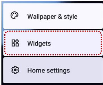
Figure 32 Widget menu
