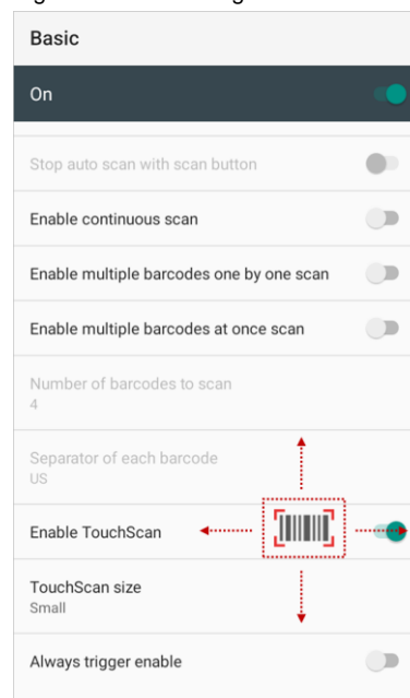
Figure 55 ScanSettings - TouchScan
