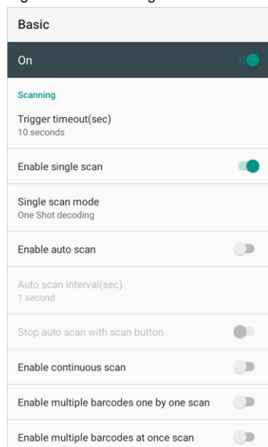
Figure 54 ScanSettings - Basic
